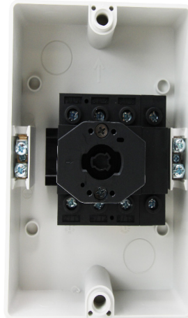
External Fixing Parts
